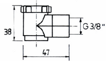
eccentric cam hollow cone-type female thread 3/8" (standard)
